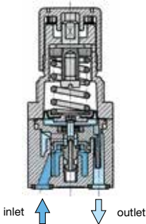
cross-section
